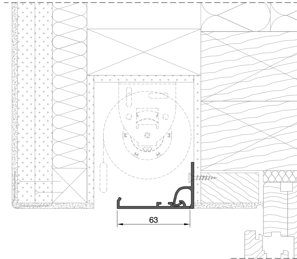
Safety hinge with cover plate 63 mm
