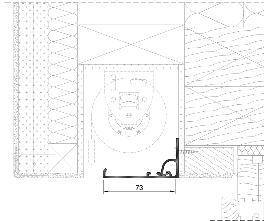
Safety hinge with cover plate 73 mm
