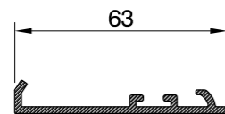
Cover plate 63 mm (art. nr. 80014)
