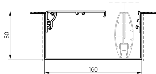
HEM BAR BOX C160x80SS (OPTIONAL)
